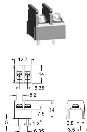
T30MRS11-02
