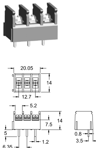
T30MBS11-03
