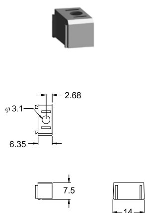
T30M-R01
