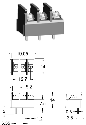
T30MRS11-03
