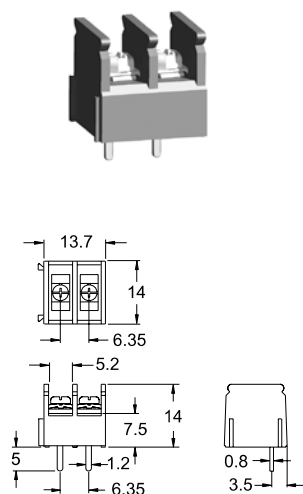
T30MBS11-02
